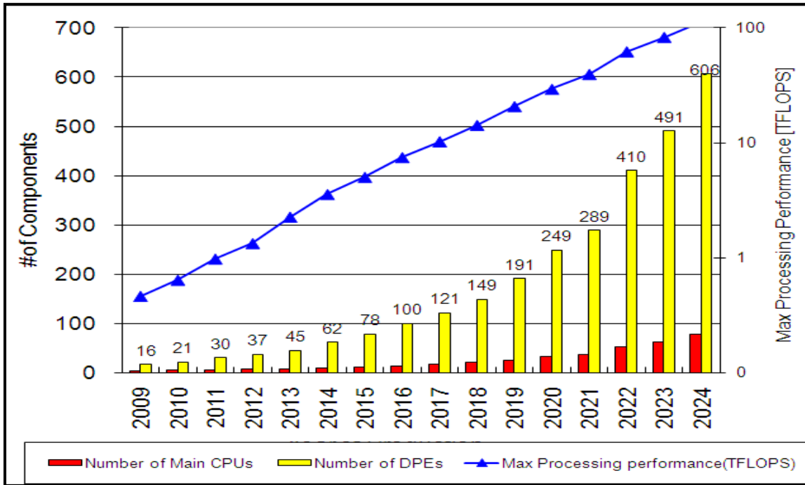
Figure SYSD9 SOC Consumer Stationary Design Complexity Trends—UPDATED
