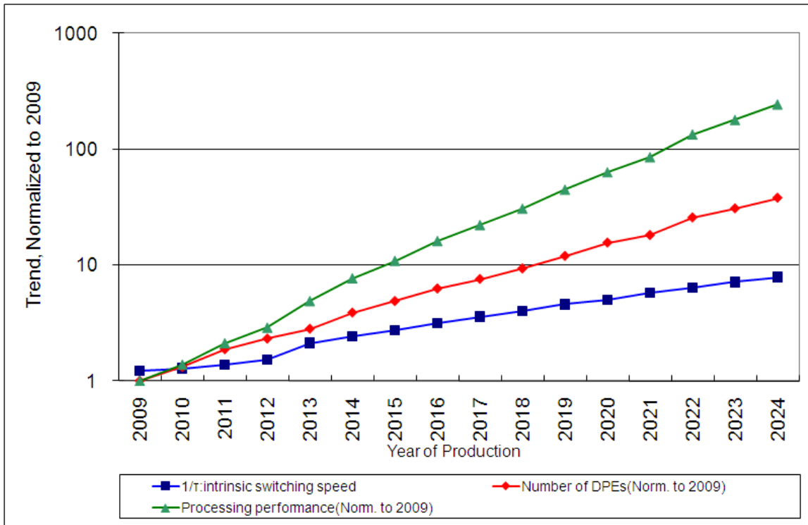
Figure SYSD10 SOC Consumer Stationary Performance Trends—UPDATED
