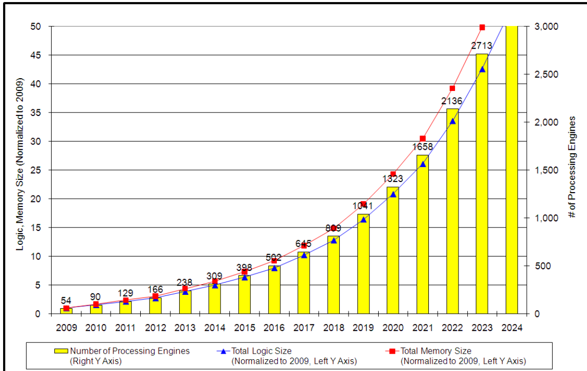
Figure SYSD5 SOC Consumer Portable Design Complexity Trends—UPDATED
