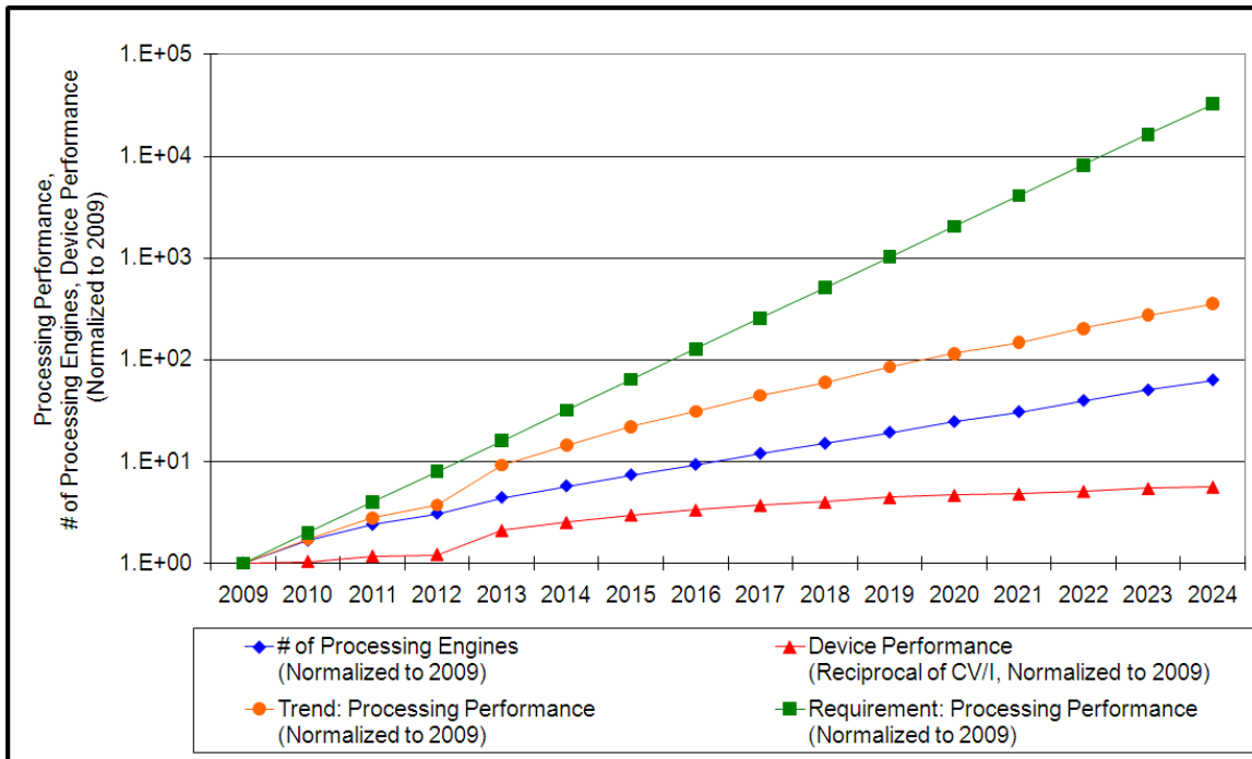
Figure SYSD7 SOC Consumer Portable Processing Performance Trends—UPDATED
