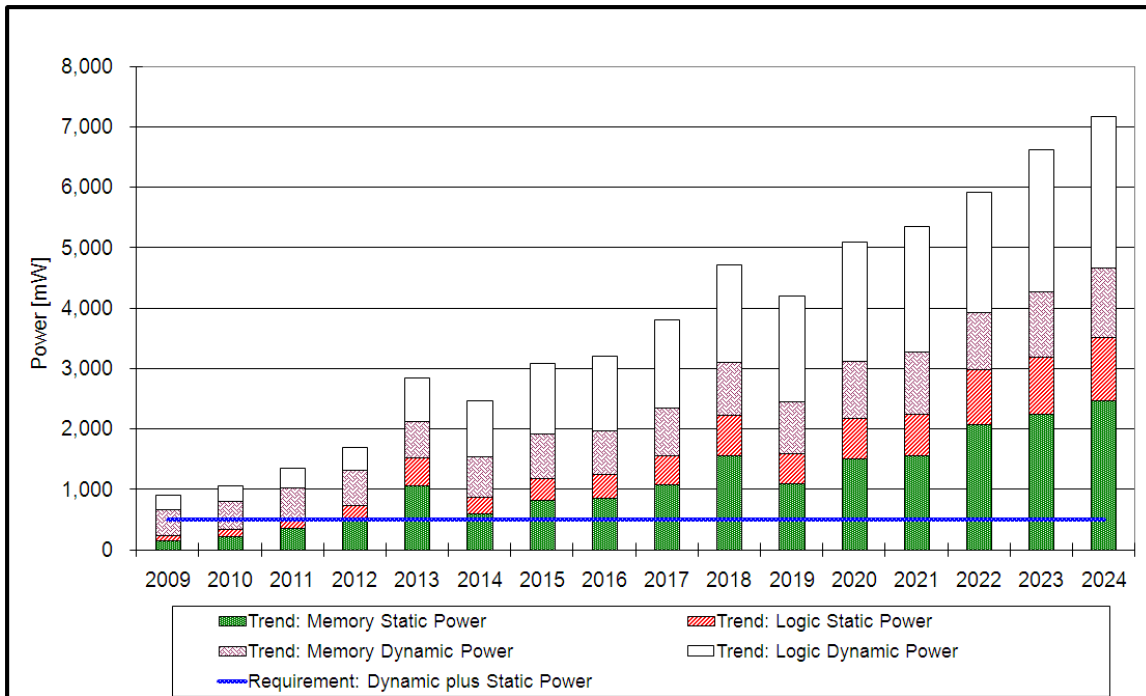
Figure SYSD6 SOC Consumer Portable Power Consumption Trends—UPDATED
